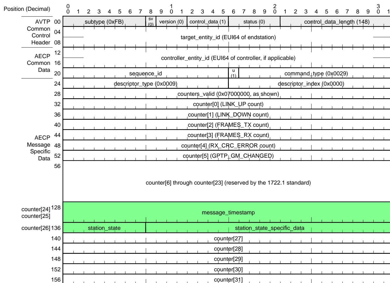
43 44 Figure 1: The Test Status Message
